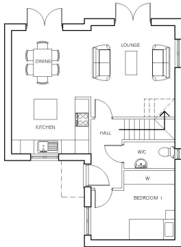
GROUND FLOOR PLAN PLOT 15
