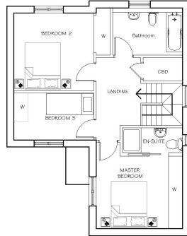
FIRST FLOOR PLAN PLOT 15
